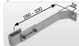
Fig. Order No. 60023, 62023, 64023
