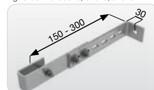
Fig. Order No. 60019, 62019, 64019
